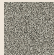
STRATUS
