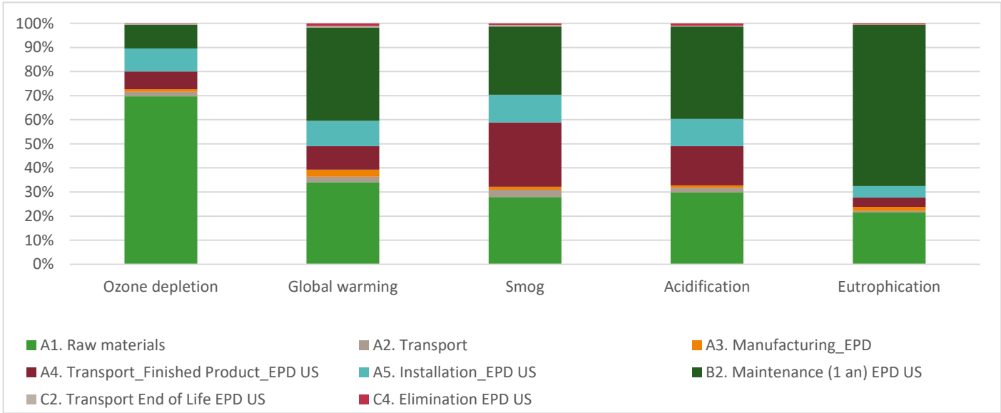
Figure 5: Graph depicting the impact indicators as calculated by the TRACI method
