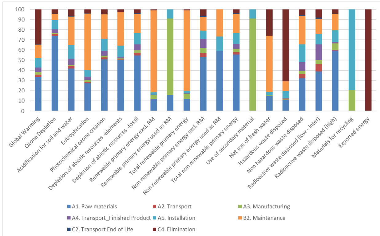
Figure 7: Graph depicting selection of impact indicator results calculated according to EN 15804 – US
